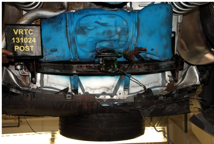
Figure 10 – Test #2 Post-test target vehicle fuel tank close-up view with hitch-receiver
