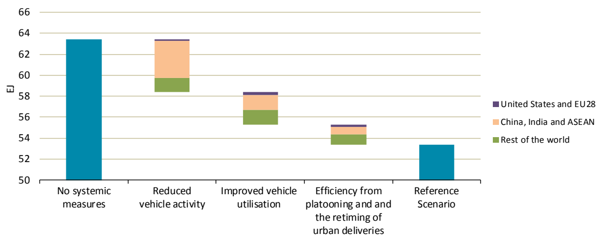
Figure 31 • Contribution to energy use reductions from measures to improve efficiency in the Reference Scenario
