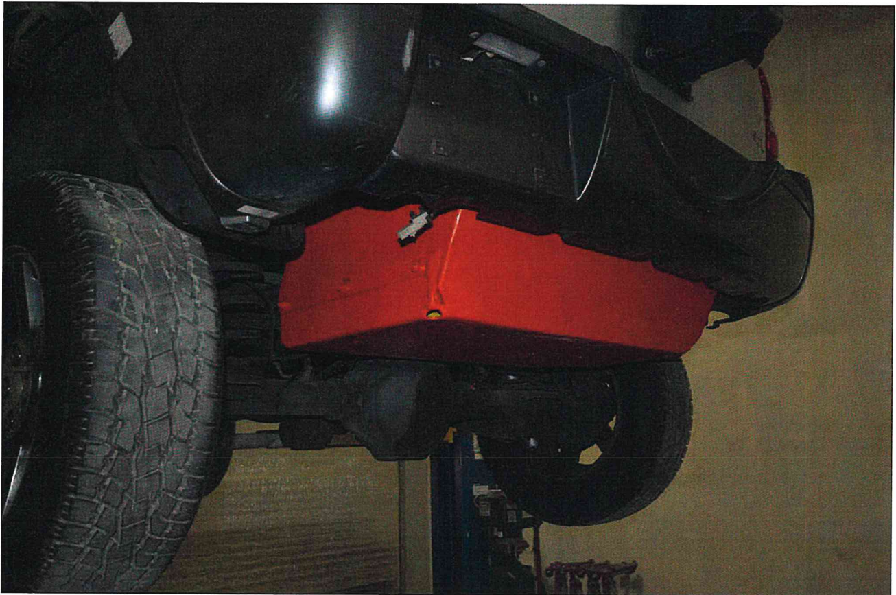
Pictorial presentation/review of the mock-up, fabrication/construction, and installation process of the FTEP onto a typical Jeep Liberty KJ
