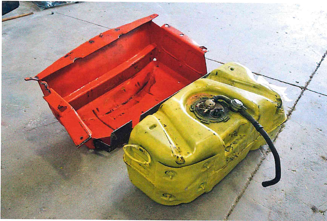
FIGURE 143. Post-Test Fuel Tank Inspection
