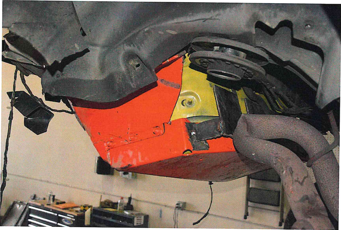
FIGURE 114. Post-Test Fuel Tank Inspection
