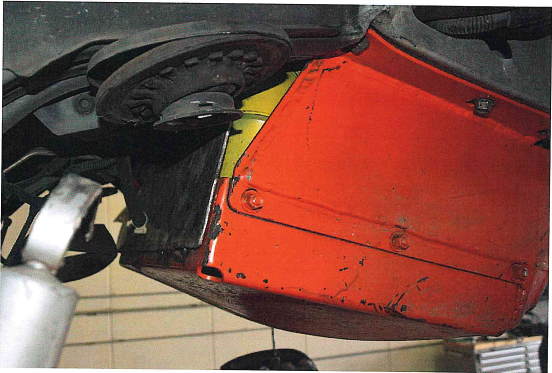
FIGURE 107. Post-Test Fuel Tank Inspection
