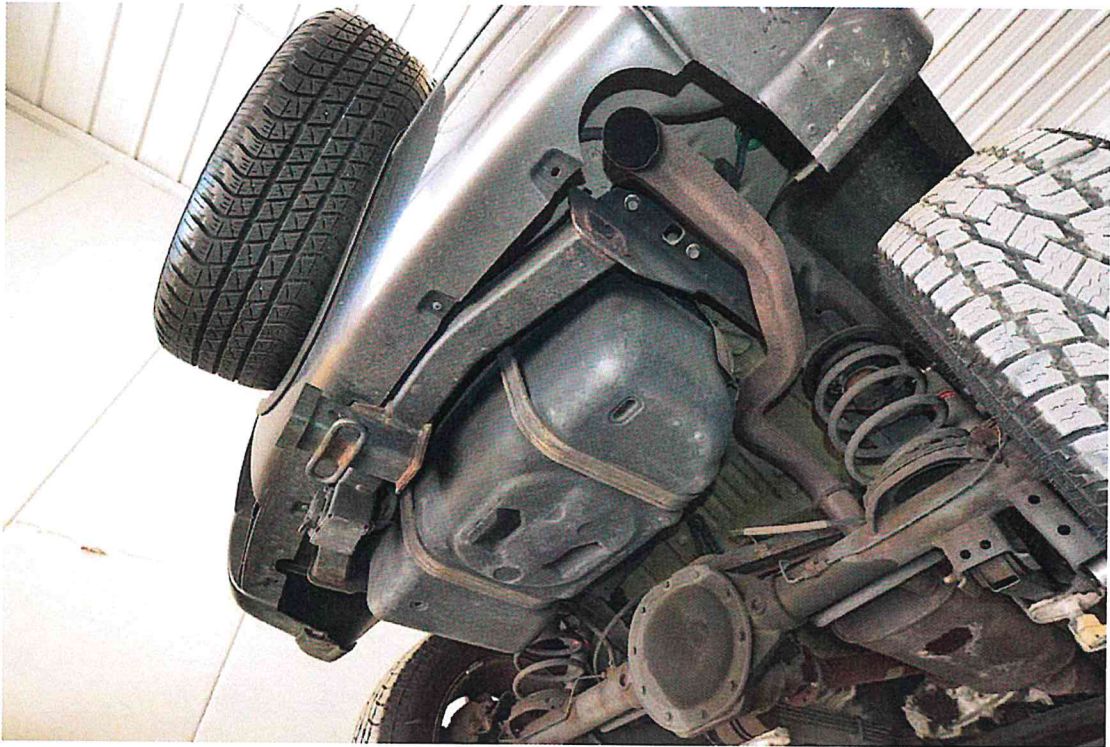
FIGURE 12. Pre-Test 2003 Jeep Liberty Fuel Tank
