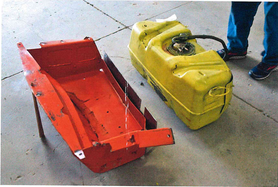
FIGURE 141. Post-Test Fuel Tank Inspection
