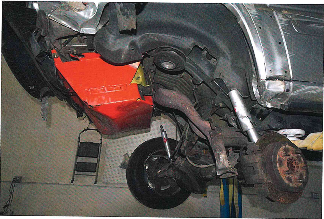
FIGURE 113. Post-Test Fuel Tank Inspection
