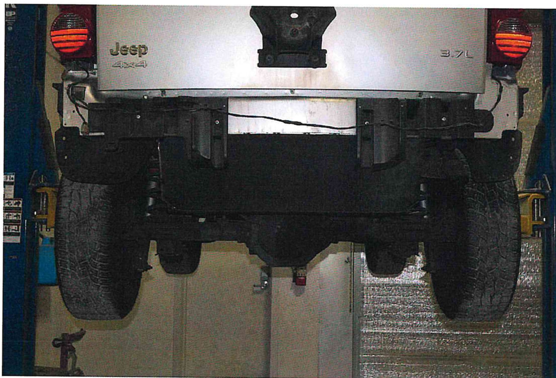
FIGURE 49. 2003 Jeep Liberty Fuel Tank Encapsulation Prototype Design Process
