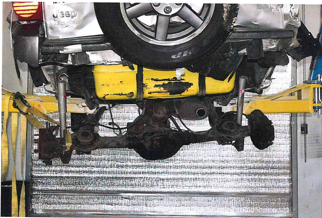
FIGURE 128. Post-Test Fuel Tank Inspection
