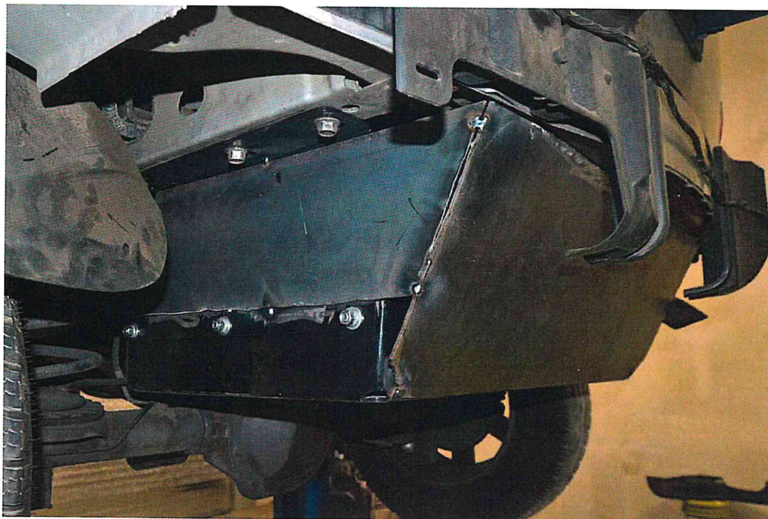
FIGURE 48. 2003 Jeep Liberty Fuel Tank Encapsulation Prototype Design Process
