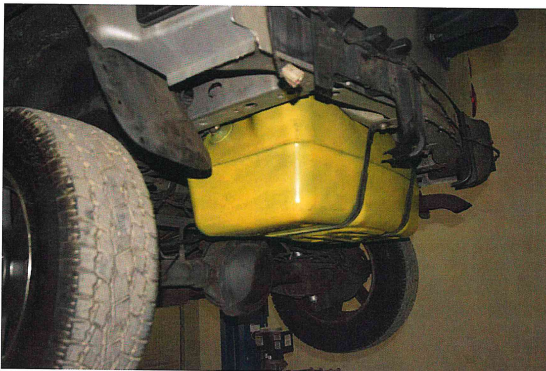
FIGURE 54. 2003 Jeep Liberty with Fuel Tank Re-Installed
