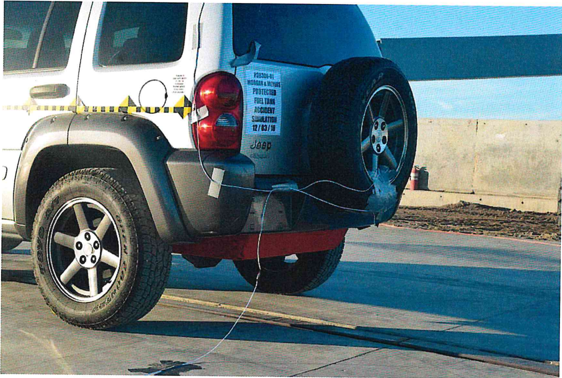
FIGURE 93. Pre-Test 2003 Jeep Liberty
