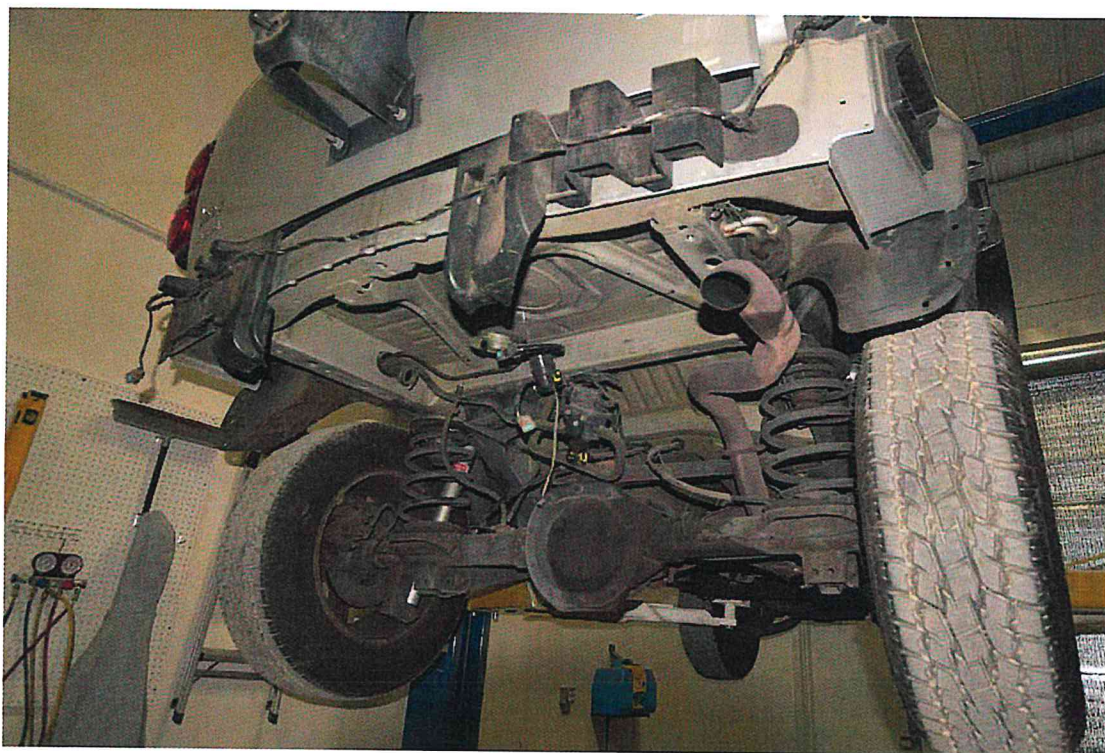
FIGURE 41. 2003 Jeep Liberty with Fuel Tank Removed
