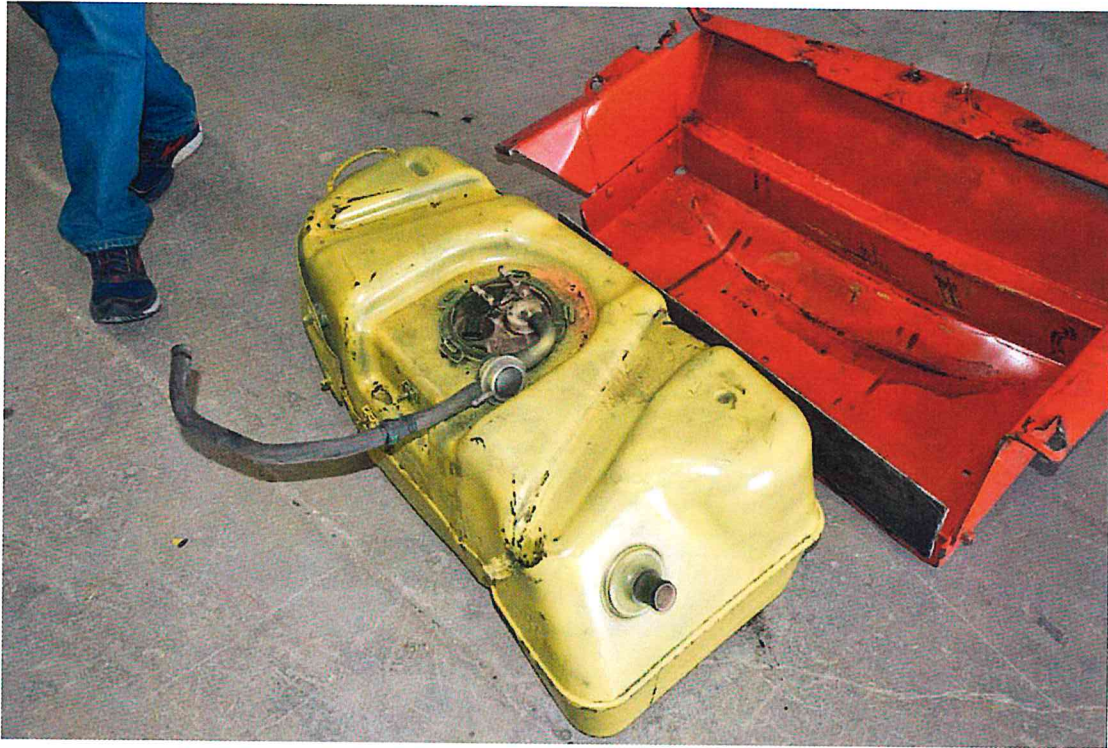
FIGURE 145. Post-Test Fuel Tank Inspection
