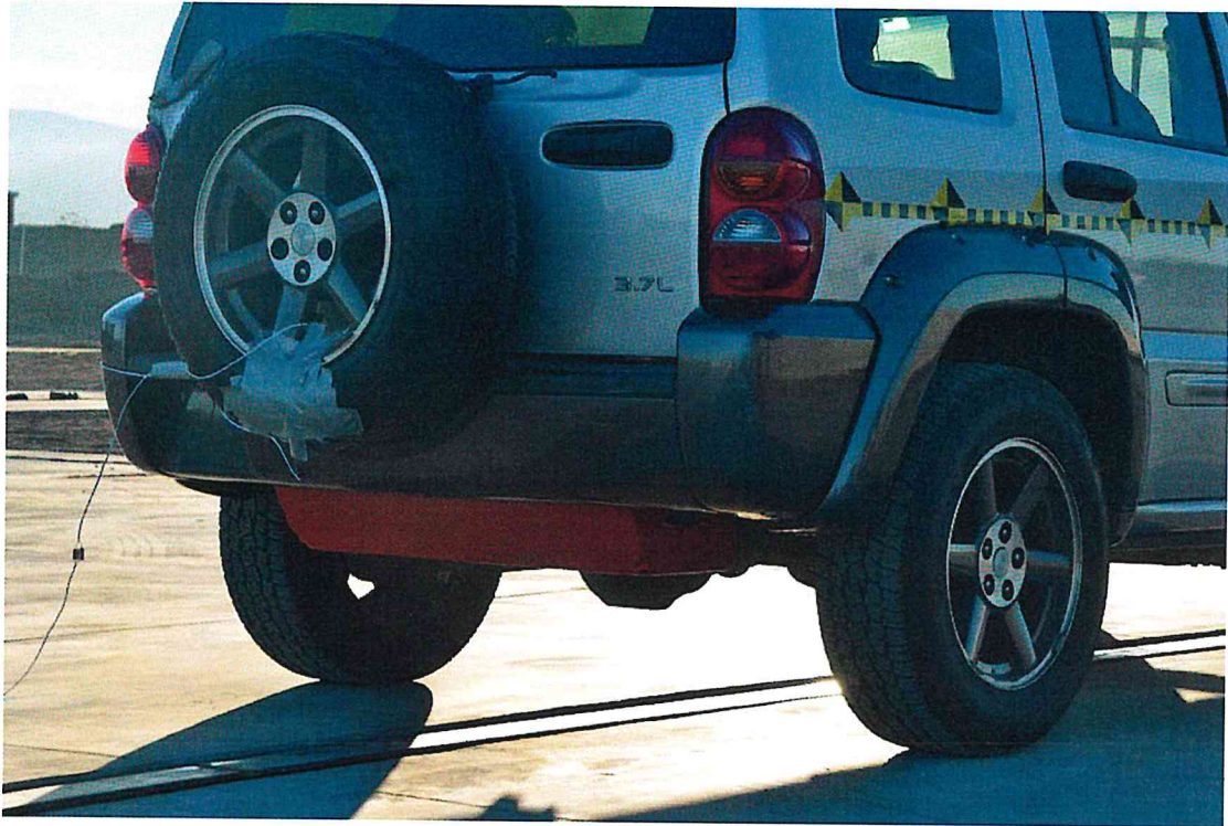
FIGURE 97. Pre-Test 2003 Jeep Liberty
