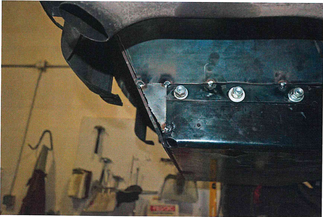
FIGURE 52. 2003 Jeep Liberty Fuel Tank Encapsulation Prototype Design Process
