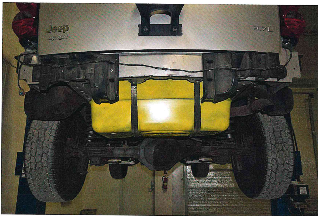
FIGURE 55. 2003 Jeep Liberty with Fuel Tank Re-Installed
