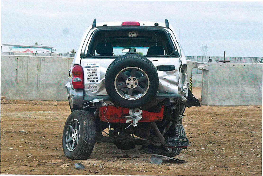
FIGURE 90. Post-Test 2003 Jeep Liberty
