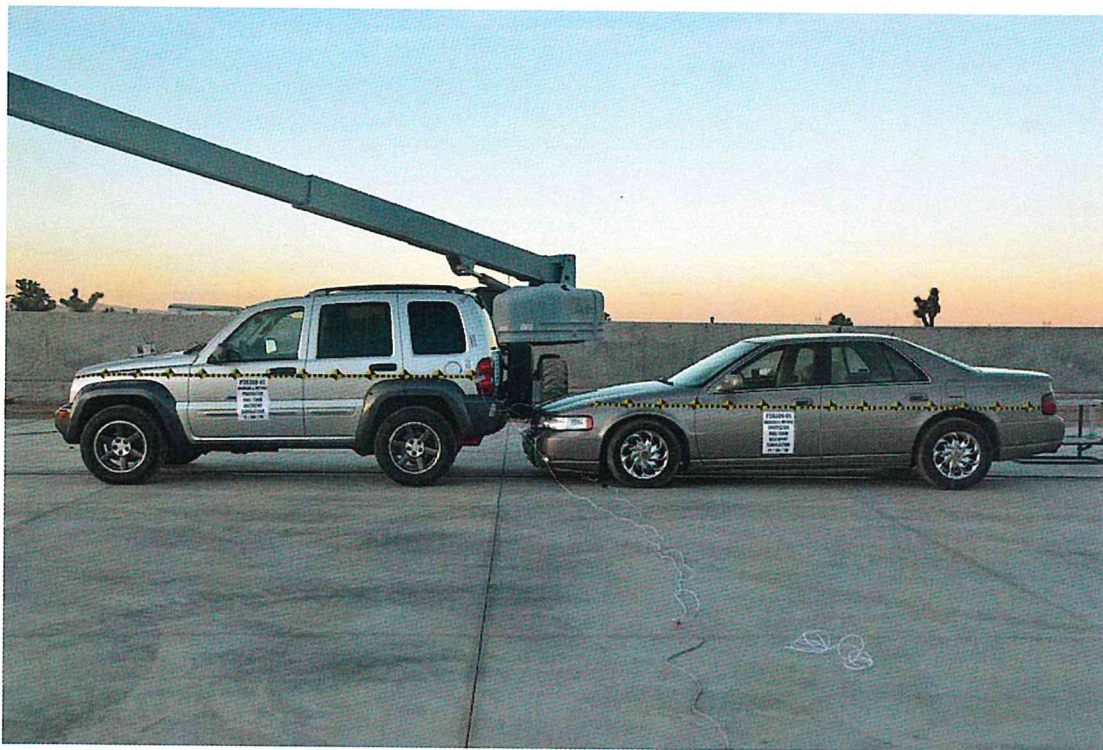
FIGURE 67. Pre-Test 2003 Jeep Liberty and 2002 Cadillac Seville SLS
