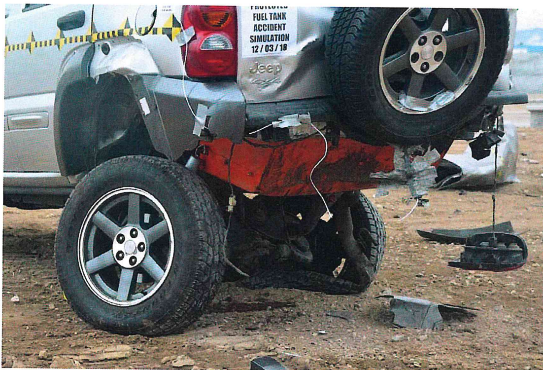
FIGURE 104. Post-Test 2003 Jeep Liberty
