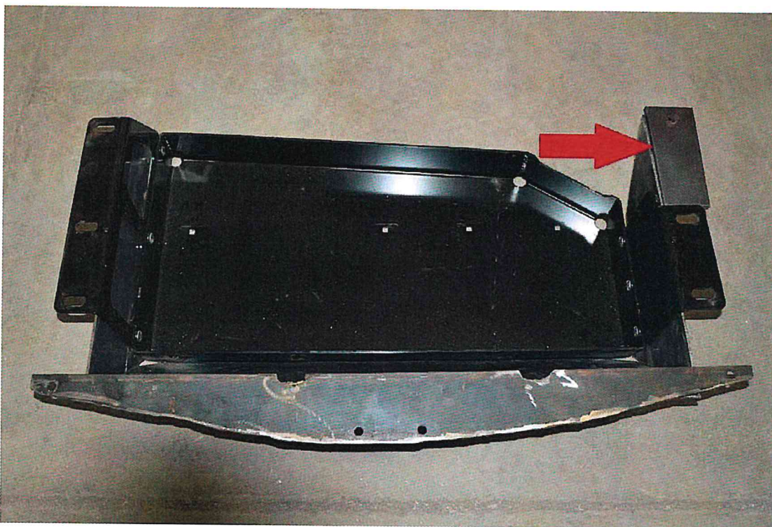
FIGURE 53. 2003 Jeep Liberty Fuel Tank Encapsulation Prototype Design Process Showing 1/2" Plate
