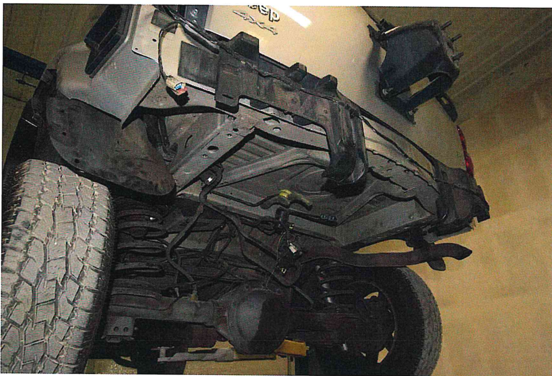
FIGURE 39. 2003 Jeep Liberty with Fuel Tank Removed
