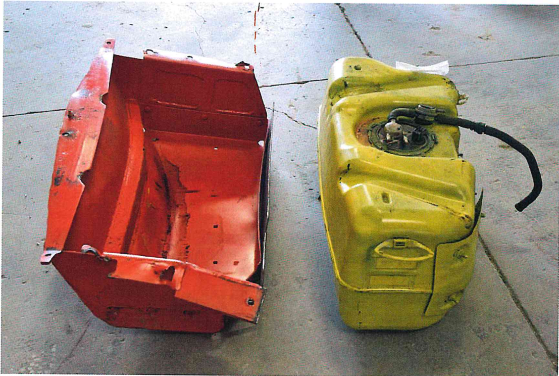
FIGURE 142. Post-Test Fuel Tank Inspection
