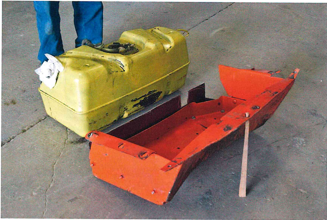
FIGURE 139. Post-Test Fuel Tank Inspection
