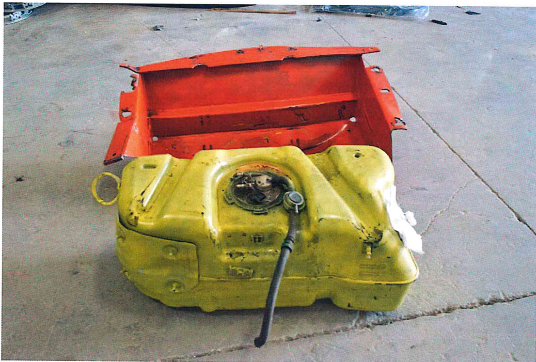
FIGURE 144. Post-Test Fuel Tank Inspection
