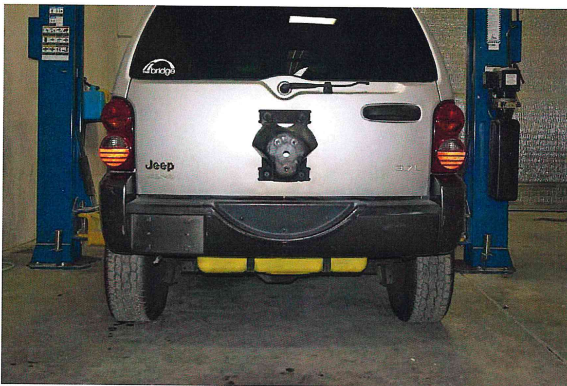
FIGURE 57. 2003 Jeep Liberty with Fuel Tank Re-Installed
