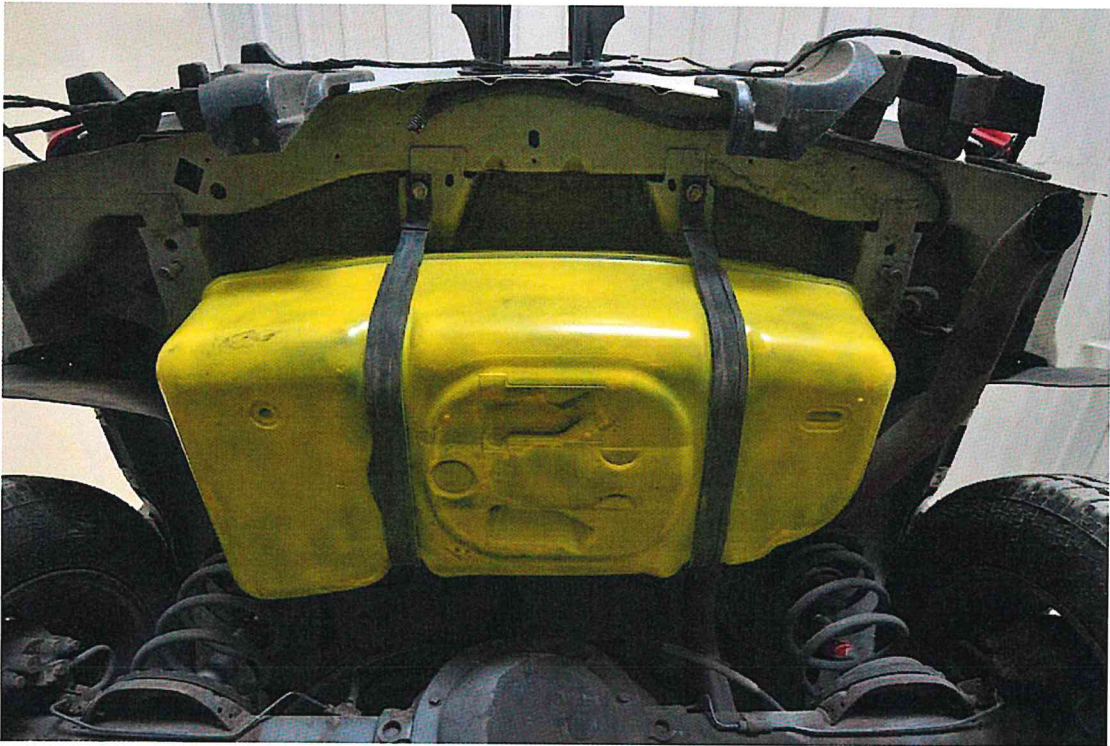
FIGURE 31. 2003 Jeep Liberty with Fuel Tank Reinstalled
