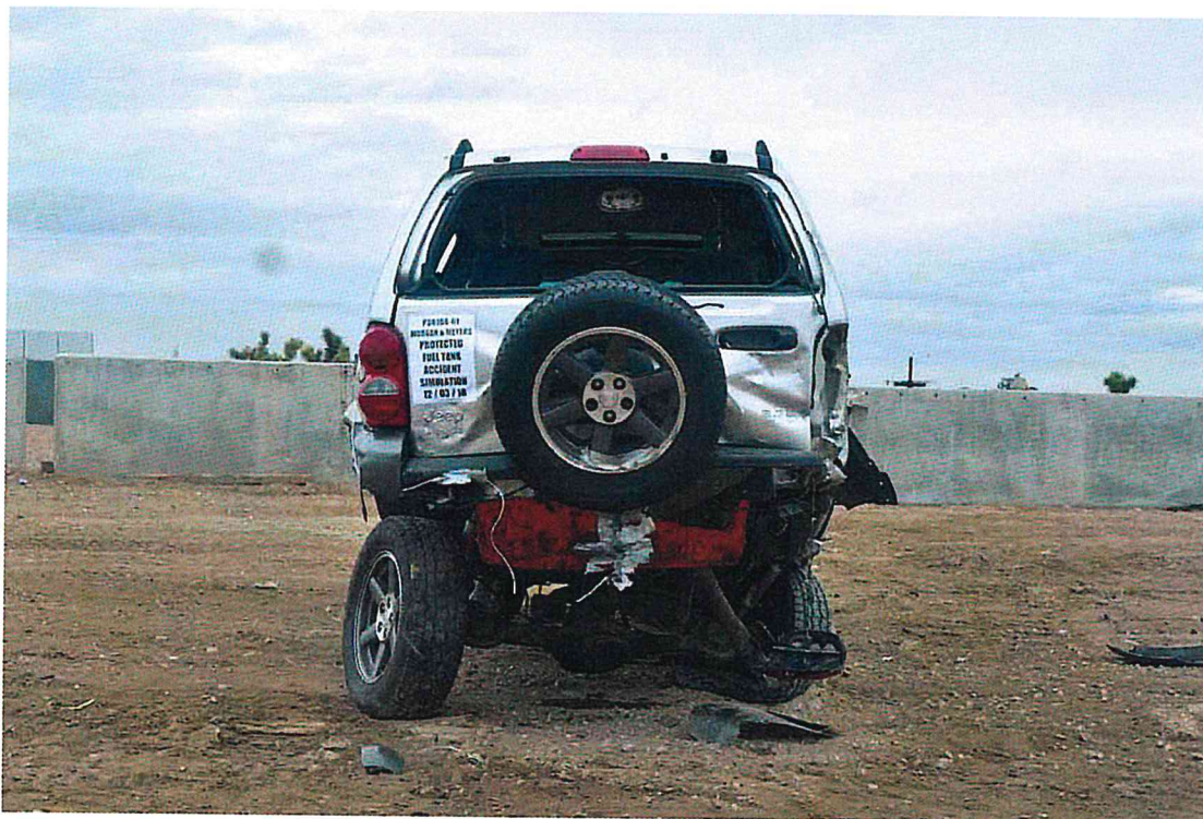
FIGURE 103. Post-Test 2003 Jeep Liberty
