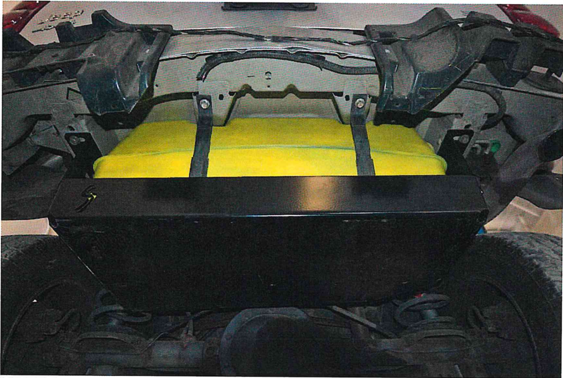
FIGURE 37. 2003 Jeep Liberty with SFK Manufacturing Model JP-4002 Skid Plate Installed
