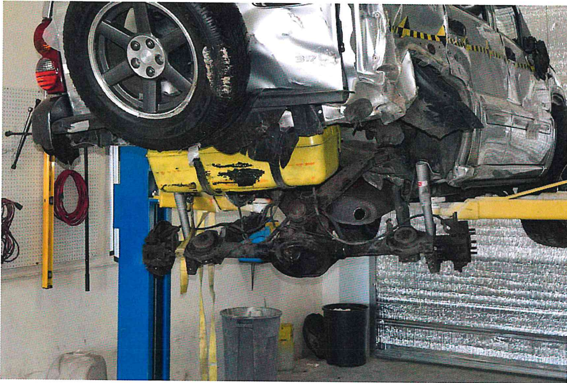
FIGURE 129. Post-Test Fuel Tank Inspection
