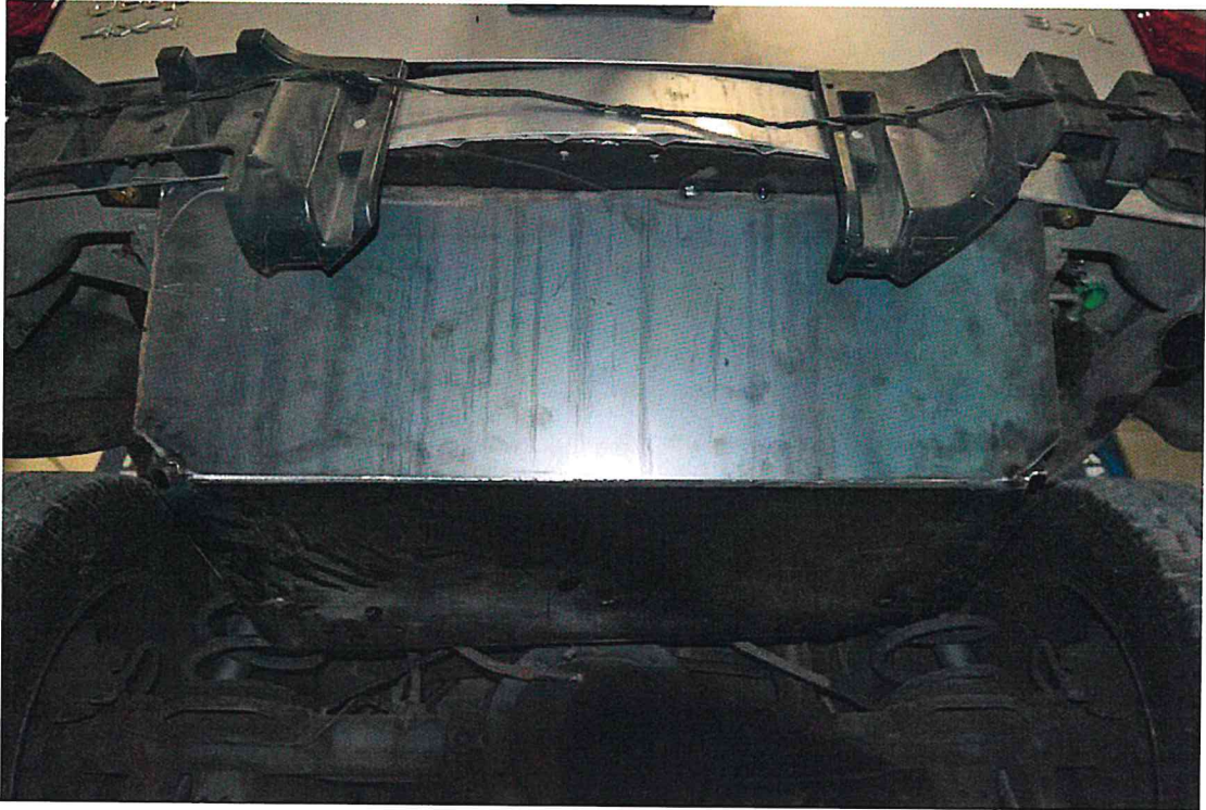
FIGURE 46. 2003 Jeep Liberty Fuel Tank Encapsulation Prototype Design Process
