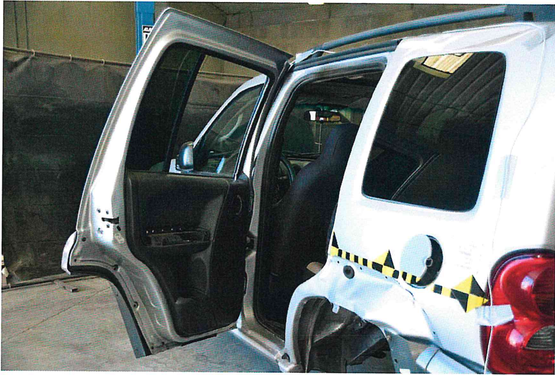
FIGURE 147. Post-Test Door Opening
