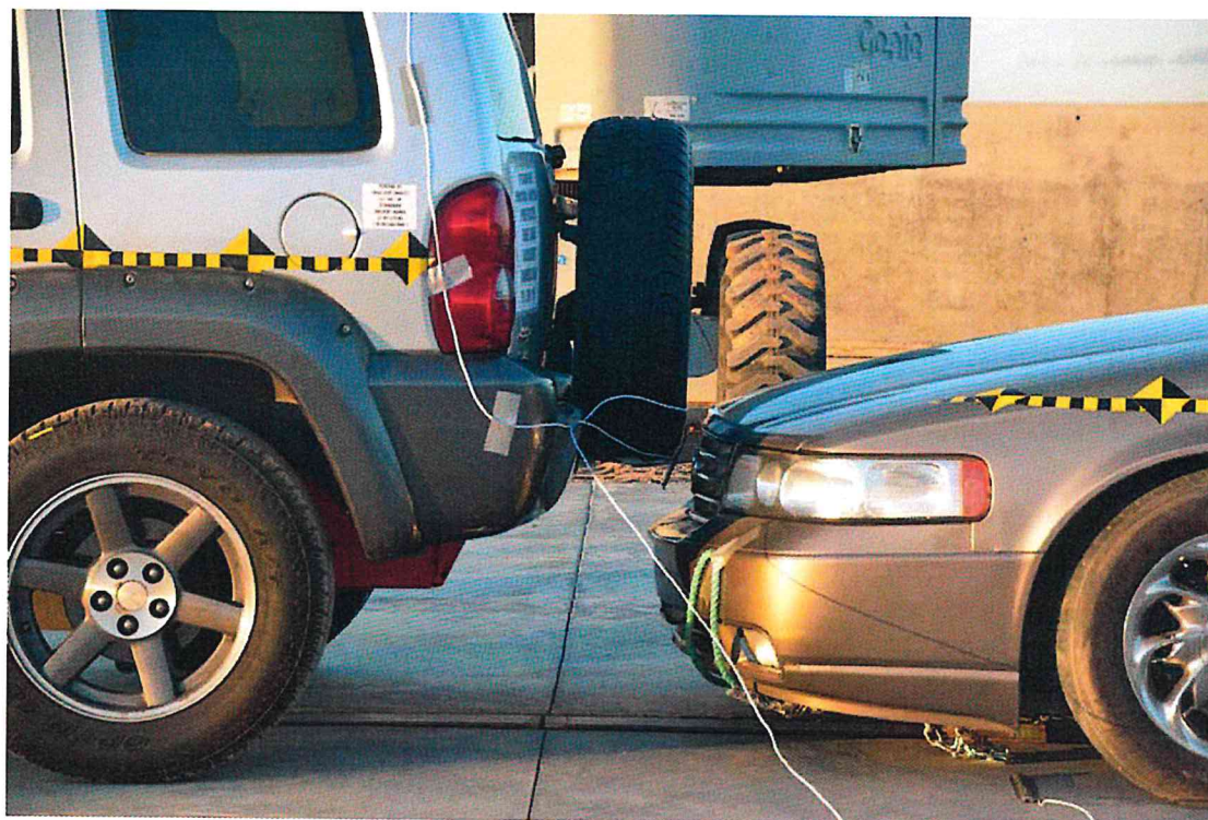
FIGURE 70. Pre-Test 2003 Jeep Liberty and 2002 Cadillac Seville SLS
