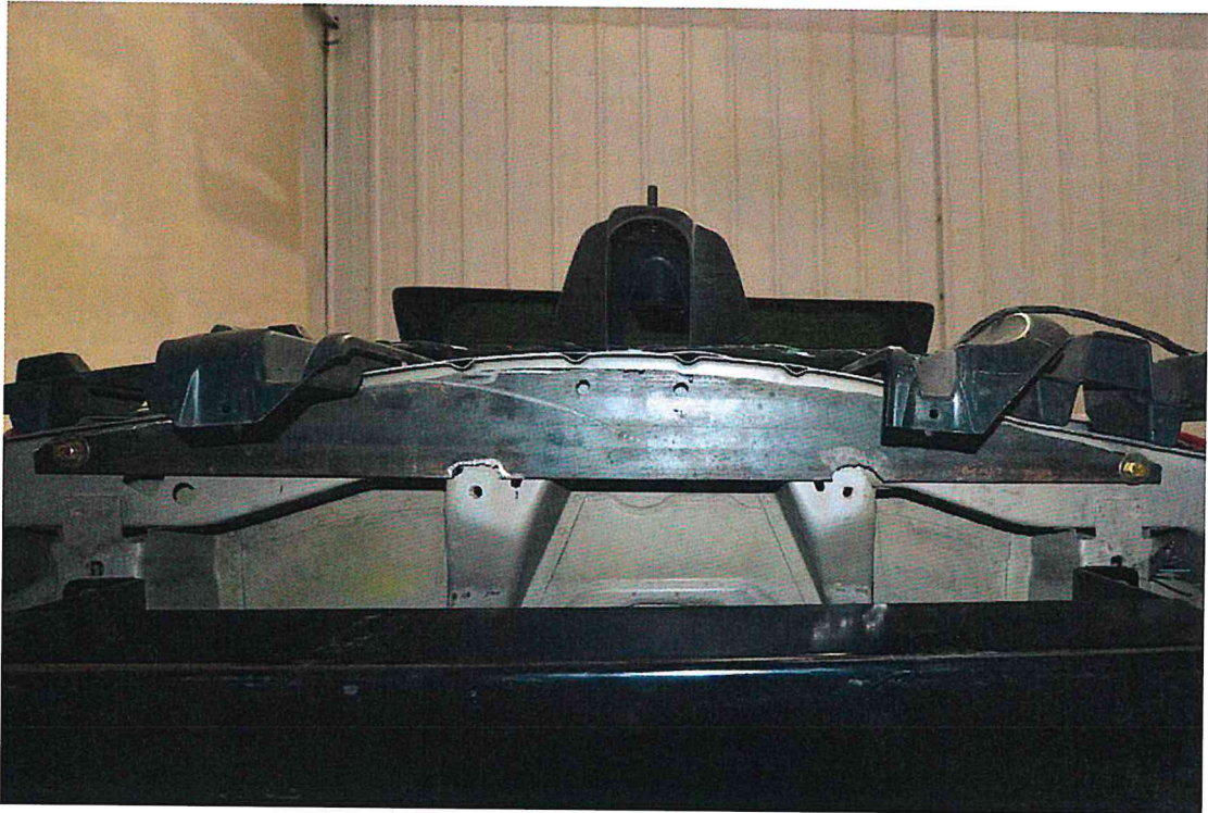
FIGURE 43. 2003 Jeep Liberty Fuel Tank Encapsulation Prototype Design Process
