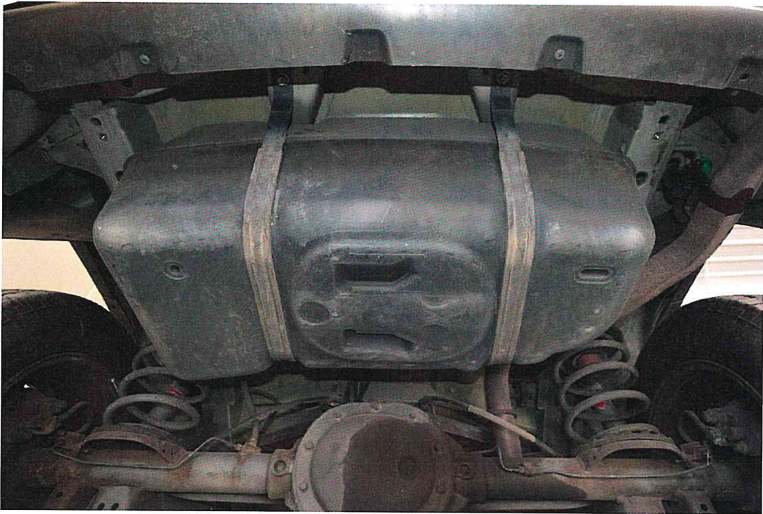
FIGURE 17. Pre-Test 2003 Jeep Liberty Fuel Tank
