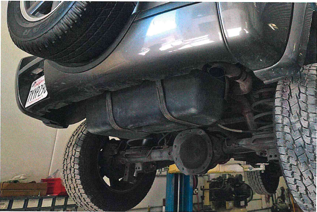
FIGURE 15. Pre-Test 2003 Jeep Liberty Fuel Tank
