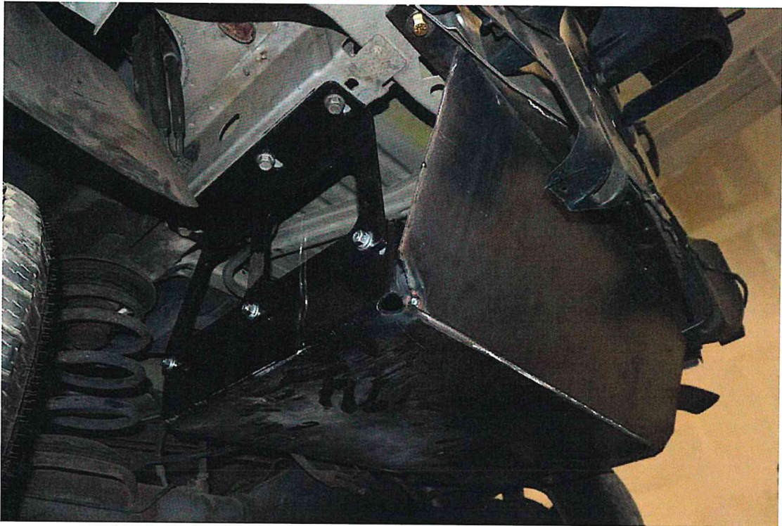
FIGURE 45. 2003 Jeep Liberty Fuel Tank Encapsulation Prototype Design Process
