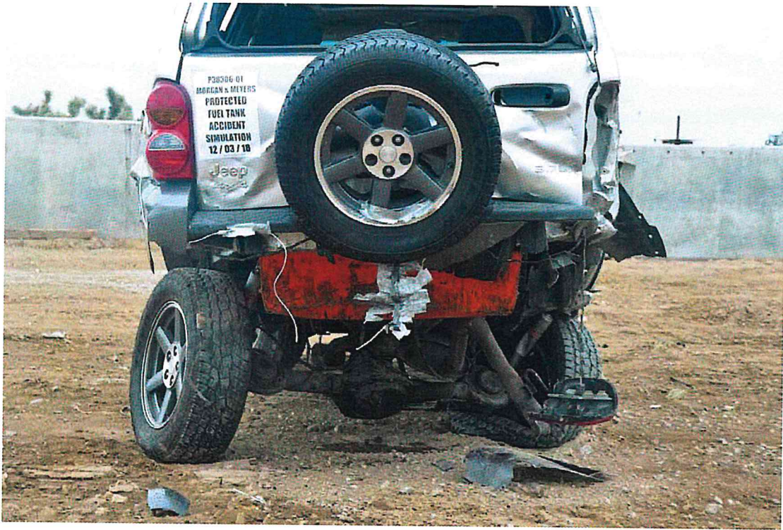
FIGURE 102. Post-Test 2003 Jeep Liberty
