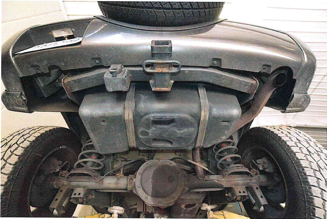
FIGURE 11. Pre-Test 2003 Jeep Liberty Fuel Tank
